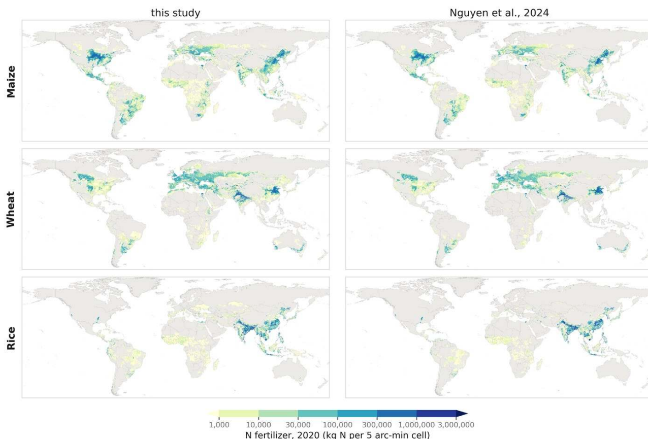
Figure S4. Grid-scale spatial comparison of maize, wheat and rice synthetic N fertilizer inputs in 2020. Global maps compare the spatial distribution of synthetic N fertilizer estimated in this study with NPKGRIDS (Nguyen et al., 2024) for maize, wheat and rice at the grid-cell level.
