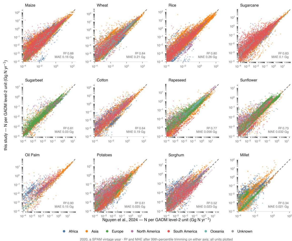
Figure S3. Second-level administrative-unit validation of crop-specific synthetic N fertilizer inputs in 2020. Comparison of synthetic N fertilizer amounts estimated in this study with NPKGRIDS (Nguyen et al., 2024) at second-level administrative units (e.g., counties, districts or comparable subdivisions) for 2020.
