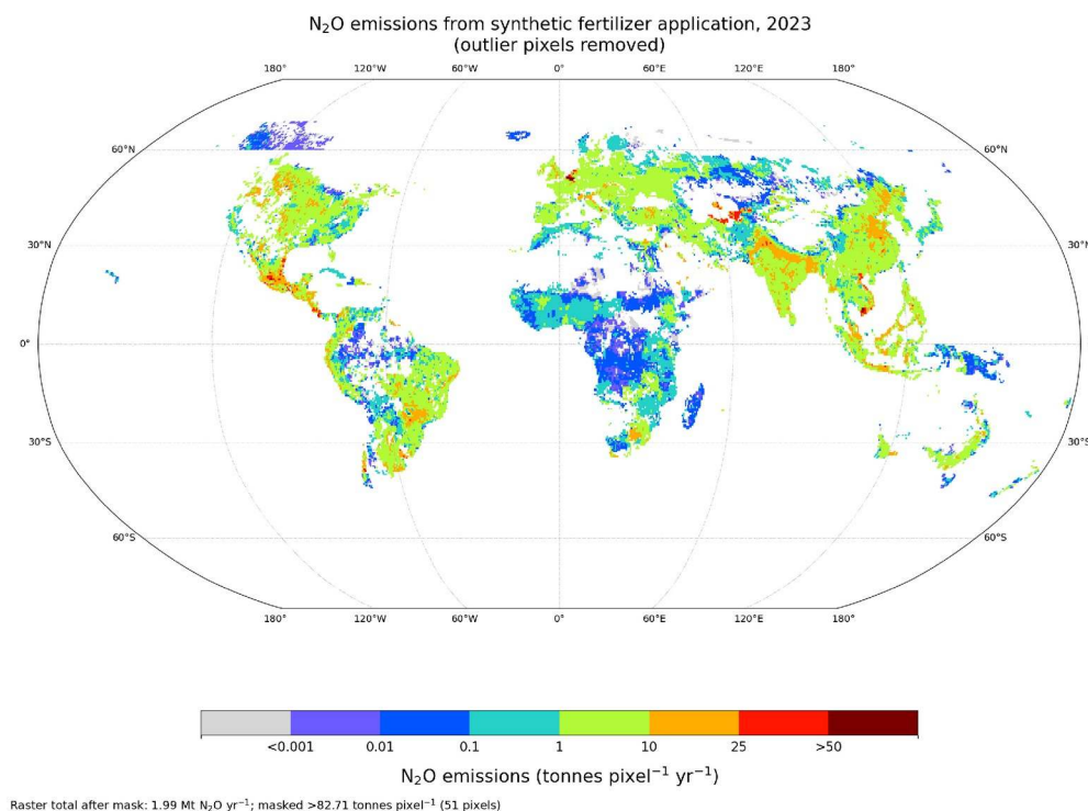
Figure 8. Global gridded distribution of N 2 O direct and indirect emissions from synthetic nitrogen fertilizer application in 2023. Emissions are expressed as tonnes of N 2 O per grid cell (pixel) per year and displayed on a logarithmic scale
