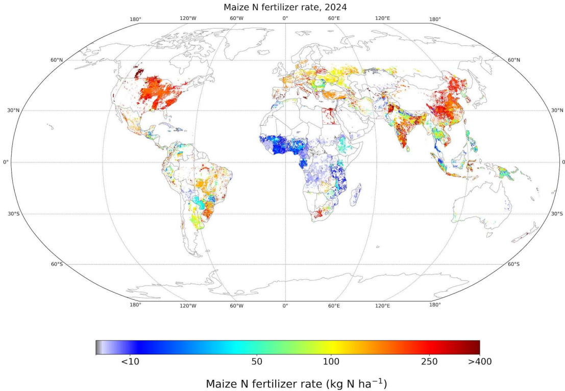
Figure 5. Example of the final gridded crop-specific synthetic N fertilizer application rate for maize in 2024.
