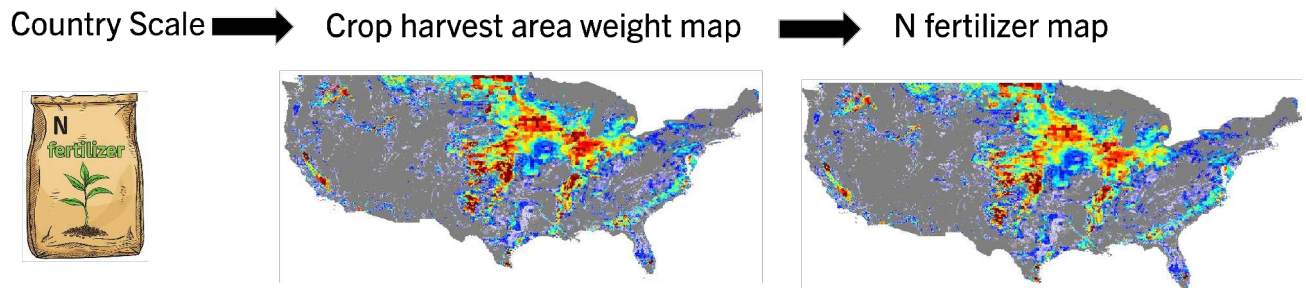
Figure 3. Example of the spatial allocation of country-level synthetic N fertilizer use to the gridded scale for the United States.
